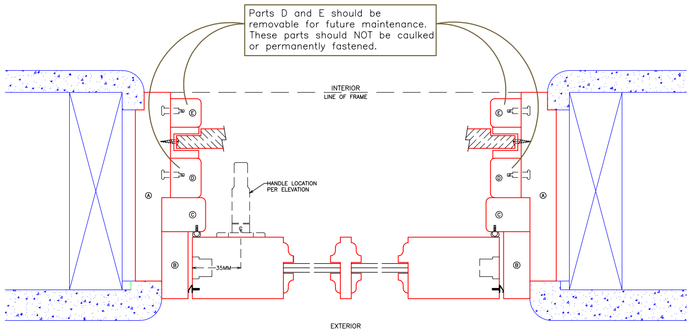
Figure 1 - Horizontal Cross Section
